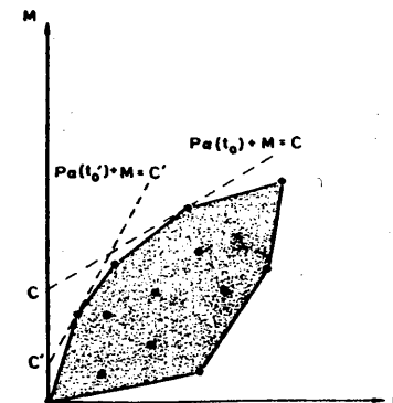
FIG. 1. Monotonicity of Payoffs in \tau_0 .
