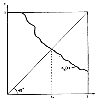
FIG. 2. Determination of x_n .
